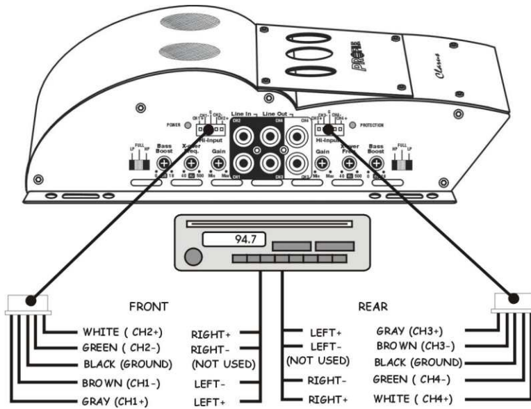
FOUR CHANNEL CONNECTIONS: FLOATING GROUND RADIO (MOST COMMON TYPE)
